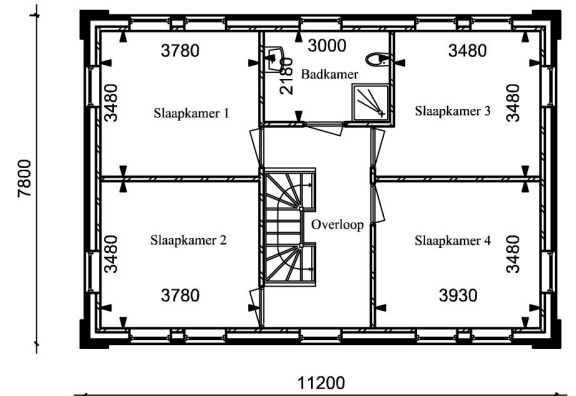
Verdieping. _____
